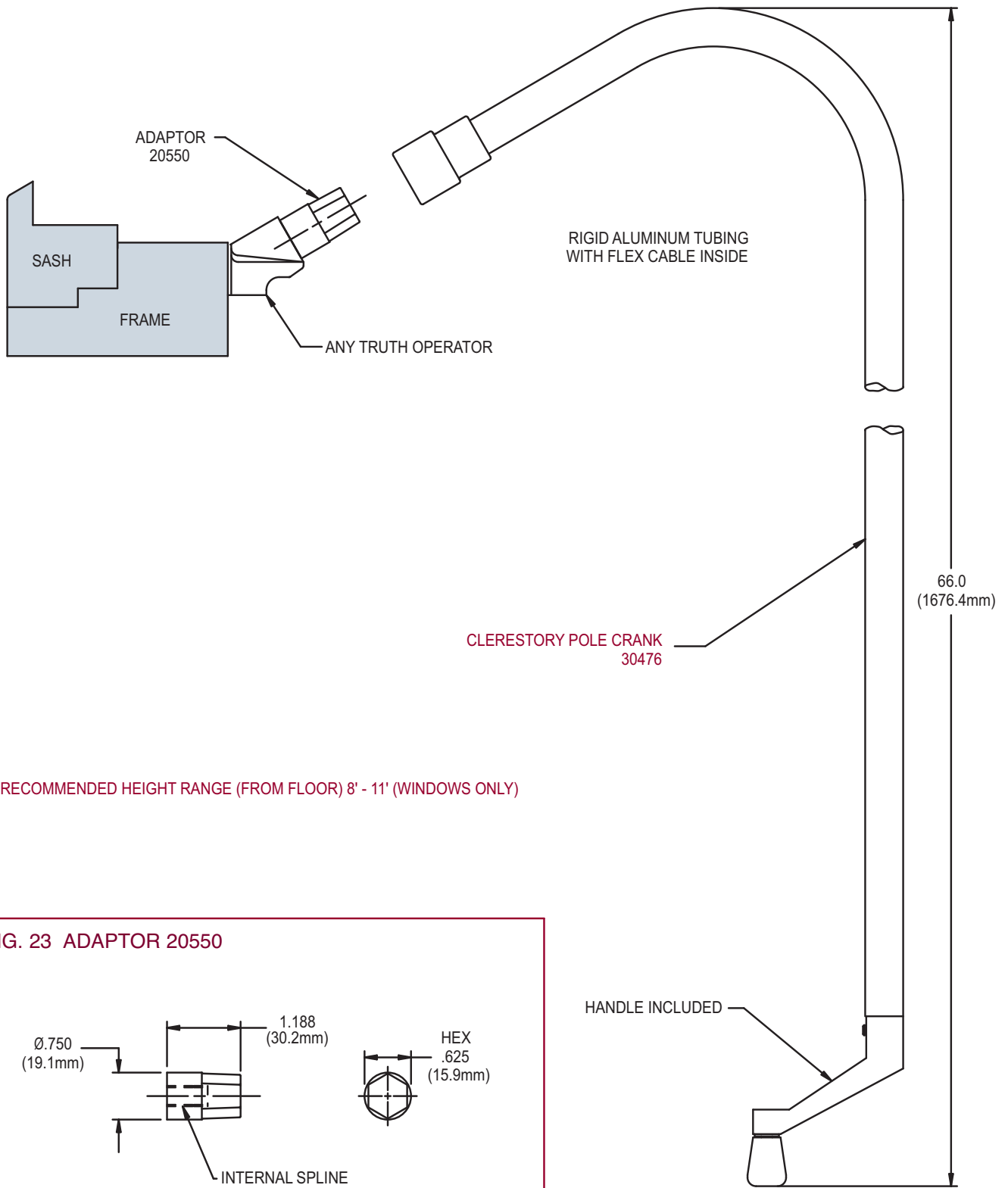
FIG. 22 APPLICATION OF CLERESTORY POLE CRANK (Not compatible with Encore)
