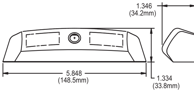
FIG. 18 METAL ENTRYGARD COVER 11328.XX (11327.XX with gasket)
