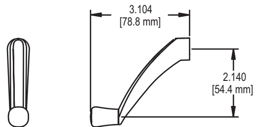
FIG. 13 CONTOUR HANDLE 11454.XX
